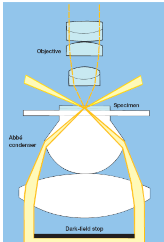
Dark-Field microscope
